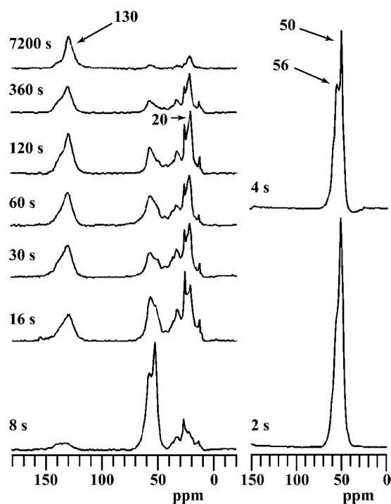
FIGURE 8. ^{13}\text{C} CP/MAS NMR spectra of samples from a pulse-quench study of methanol conversion on HSAPO-34 at 673 K. Each sample was prepared by injecting 20 \mu\text{L} of methanol- ^{13}\text{C} onto a freshly activated catalyst bed (0.3 g) while He was flowed at 600 \text{mLmin}^{-1} , and reaction occurred for the times shown followed by a rapid thermal quench.
