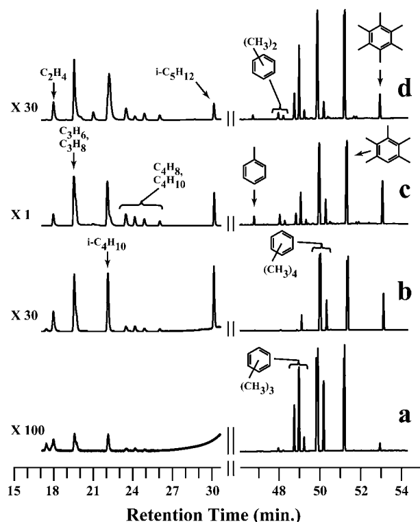
FIGURE 9. GC-MS total ion chromatograms from experiments probing the reactions of methylbenzenes either alone or with methanol- ^{13}\text{C} . All experiments shown were carried out at 723 K using HBeta with \text{SiO}_2/\text{Al}_2\text{O}_3 = 75 and gas sampling at 1.5 s. (a) Durene alone, showing a very low yield of olefins. (b) Hexamethylbenzene alone showing a modest yield of olefins. (c) Methanol- ^{13}\text{C} and toluene 5:1 (mol:mol) produced the highest yield of olefins. (d) Control experiment using water and hexamethylbenzene 5:1 (mol:mol).
