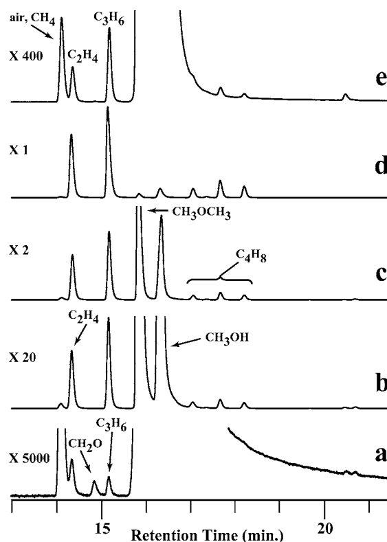
FIGURE 10. GC (FID detector) analyses of the product streams sampled 2.4 s after pulsing 12.5 \mu\text{L} methanol onto 300 mg beds of HSAPO-34 at 648 K. Samples a–d are from a single bed of rigorously calcined HSAPO-34 following a series of pulses of fractionally distilled methanol delivered in 30 min intervals. (a) Following the first pulse, the total yield of volatile hydrocarbons was ca. 26 ppm. (b) Following a second methanol pulse the yield of volatile hydrocarbon products increased to 1.5%. (c) Following a third, methanol pulse the yield further increased to 10%. (d) This catalyst bed was reacted with an additional 200 \mu\text{L} of methanol to create a larger hydrocarbon pool. 30 min later another 12.5 \mu\text{L} methanol pulse gave nearly complete conversion. (e) Following the first pulse of fractionally distilled methanol onto a fresh HSAPO-34 bed prepared using the standard calcination procedure but not the more rigorous second calcination. The volatile hydrocarbon yield, 590 ppm, was substantially higher without rigorous calcination, cf. (a).
