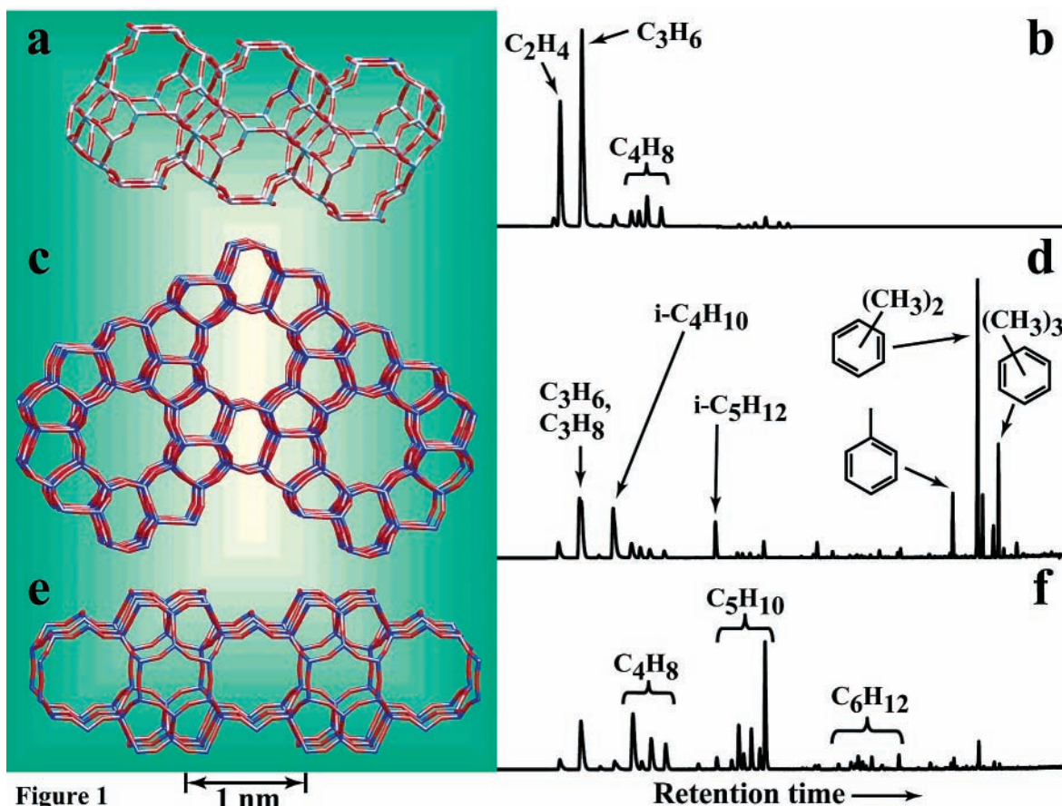
FIGURE 1. Three of the methanol conversion catalysts discussed in this contribution and GC-MS total ion chromatograms illustrating product selectivity on these materials: (a) The CHA topology of the silico-aluminophosphate catalyst HSAPO-34. (b) The products of methanol conversion on HSAPO-34. (c) The MFI structure of the aluminosilicate zeolite HZSM-5. (d) The products of methanol conversion on HZSM-5. (e) The FER topology of H-Ferrierite. (f) The products of methanol conversion on MTO catalysis on H-Ferrierite. Each experiment used 300 mg of catalyst operated at 723 K, and products were sampled 1.5 s following pulsed introduction of 10.2 \mu\text{L} of methanol.
