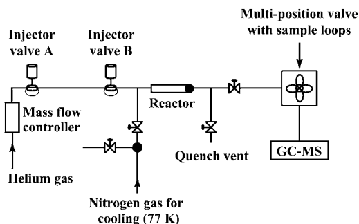
FIGURE 5. Diagram of a pulse-quench catalytic reactor used for mechanistic studies of MTO catalysis. One or more injector valves (two shown) or a syringe pump and a valve are used to treat a catalyst bed in order to prepare some transient state.
