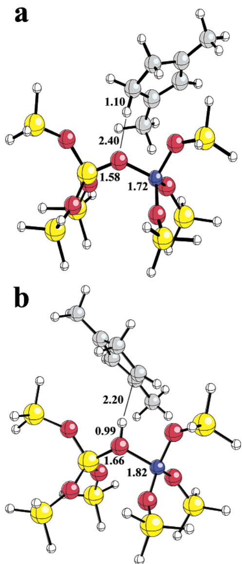
FIGURE 7. B3LYP/6-311G** optimized geometries of species on a cluster model of the acid site of HZSM-5: (a) Ion-pair complex of the 1,3-dimethylcyclopentadienyl cation 4 coordinated to the zeolite anion (ion-pair structure). (b) The \pi complex formed by the neutral cyclic diene and the zeolite acid site.
