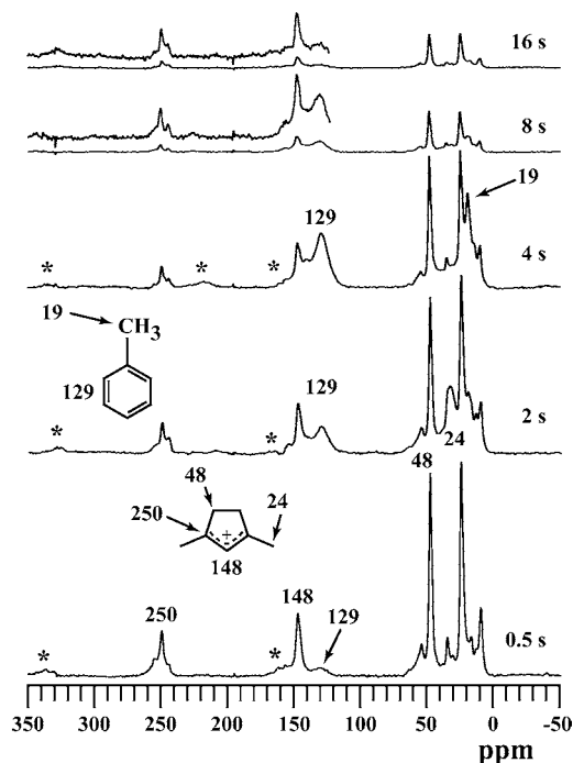
FIGURE 6. ^{13}\text{C} CP/MAS solid-state NMR spectra of the reaction products of ethylene- ^{13}\text{C}_2 forming at 623 K on zeolite HZSM-5 catalysts beds. Samples were prepared using the catalytic flow reactor in the previous figure and reaction times of 0.5–16 s.
