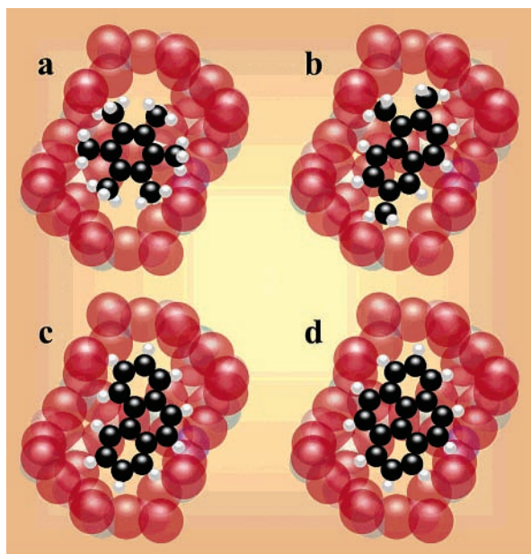
FIGURE 2. Molecular view of MTO catalyst deactivation shown for the specific case of HSAPO-34. (a) Hexamethylbenzene and other methylbenzenes are present in a few percent of cages in an active MTO catalyst. (b) With increasing time on stream, some of the methylbenzenes age into methylnaphthalenes. (c) Further aging to phenanthrene causes a loss of MTO activity in HSAPO-34. (d) The largest ring system to form in HSAPO-34 is pyrene.
